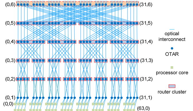
Figure 4. FONoC topology of for a 64-core MPSoC
